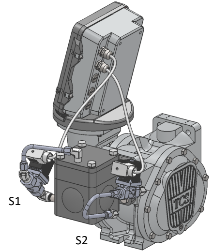
755-30 Diaphragm 3" Valve
