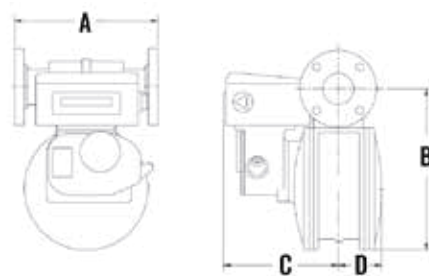
Single Capsule
