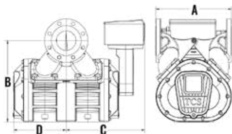
TCS 700-60SPA
