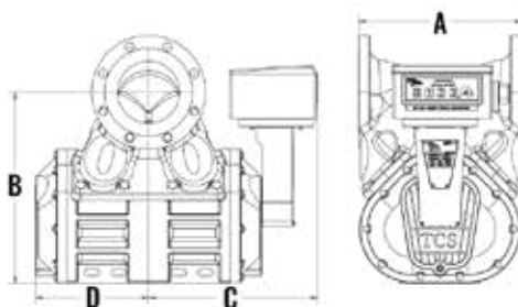
TCS 700-60/65SPA
