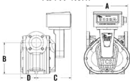
TCS 700-40SPA
