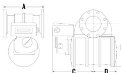
Triple Capsule
